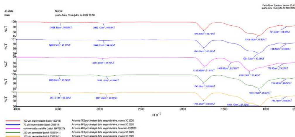
Figure 4. Fourier transform infrared (FTIR) spectrums. The FTIR spectrum showed vibrational modes typical of PTMC + PLGA (Groups 1–4) and PLG + PTMC (Group 5).
