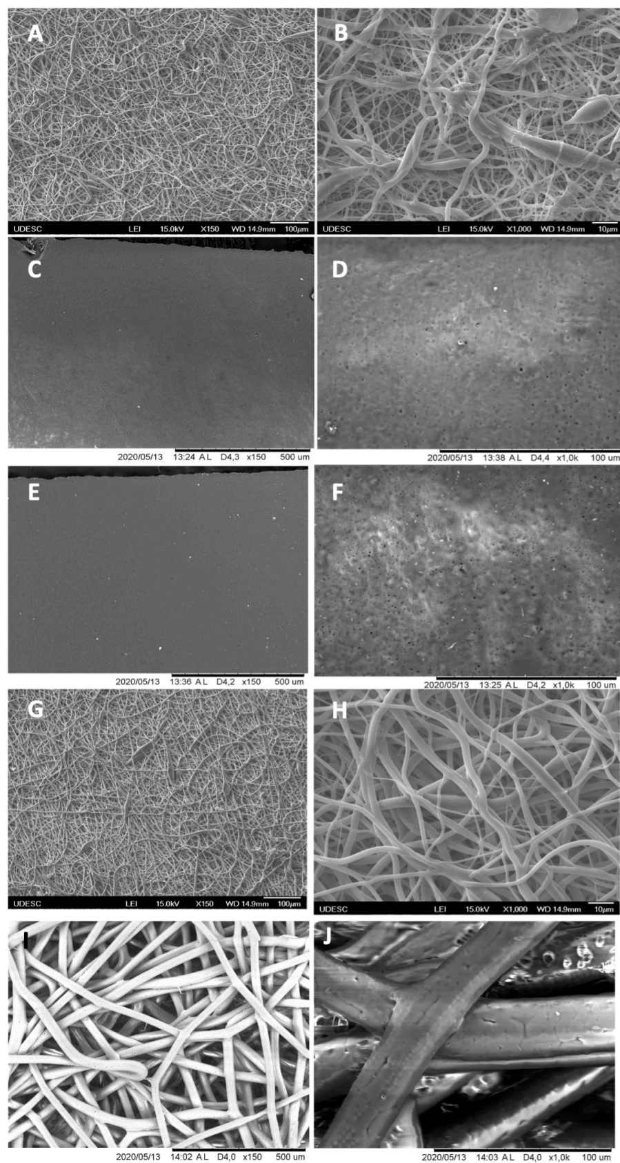
Figure 3. Scanning electron microscopy (SEM) micrographs according to the experimental groups. (A,B): Group 1; (C,D): Group 2; (E,F): Group 3; (G,H): Group 4; (I,J): Group 5. (A,C,E,G,I): 150× magnification; (B,D,F,H,J): 1000× magnification.
